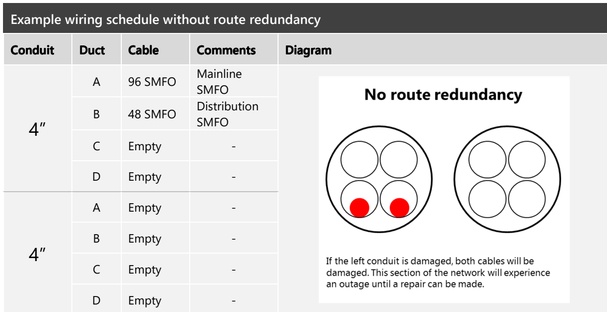
Figure 8-4: Non-redundant wiring schedule
