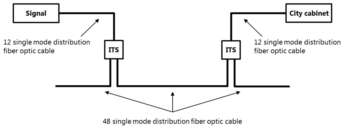
Figure 8-8: Lateral cabling
