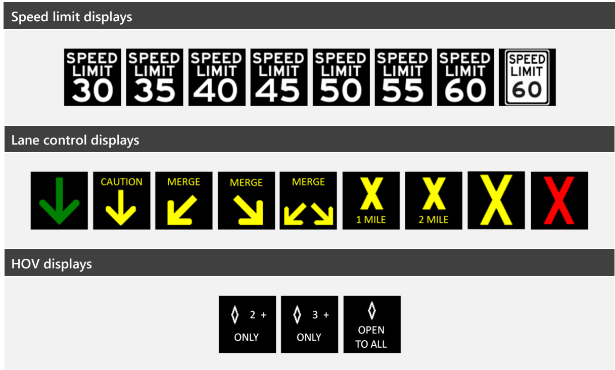
Figure 5-4: LCS displays
