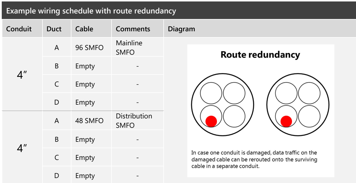
Figure 8-3: Redundant wiring schedule
