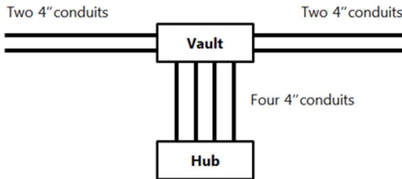
Figure 8-1: Raceways
