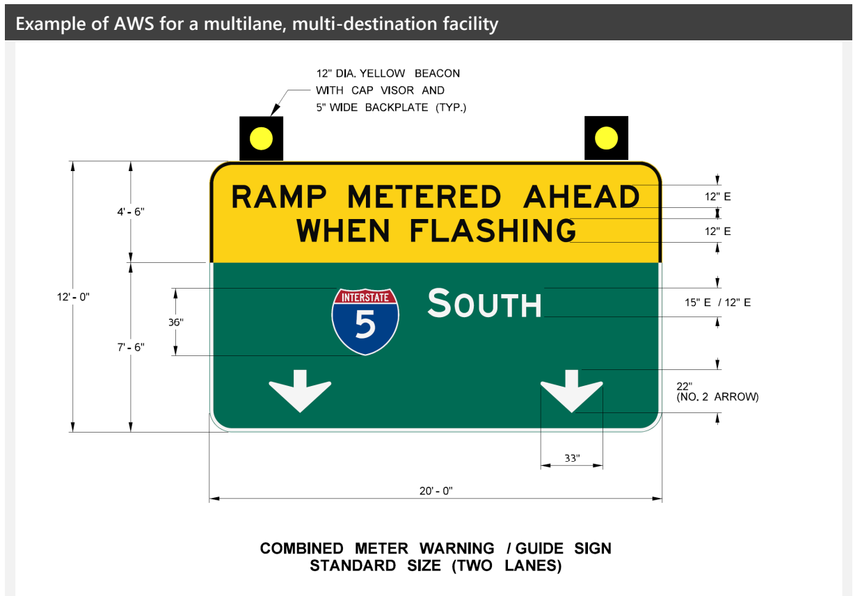
Figure 4-7: AWS for multilane, multi-destination facility
