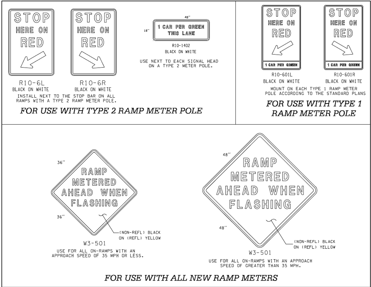
Figure 4-6: Signing for ramp meters
