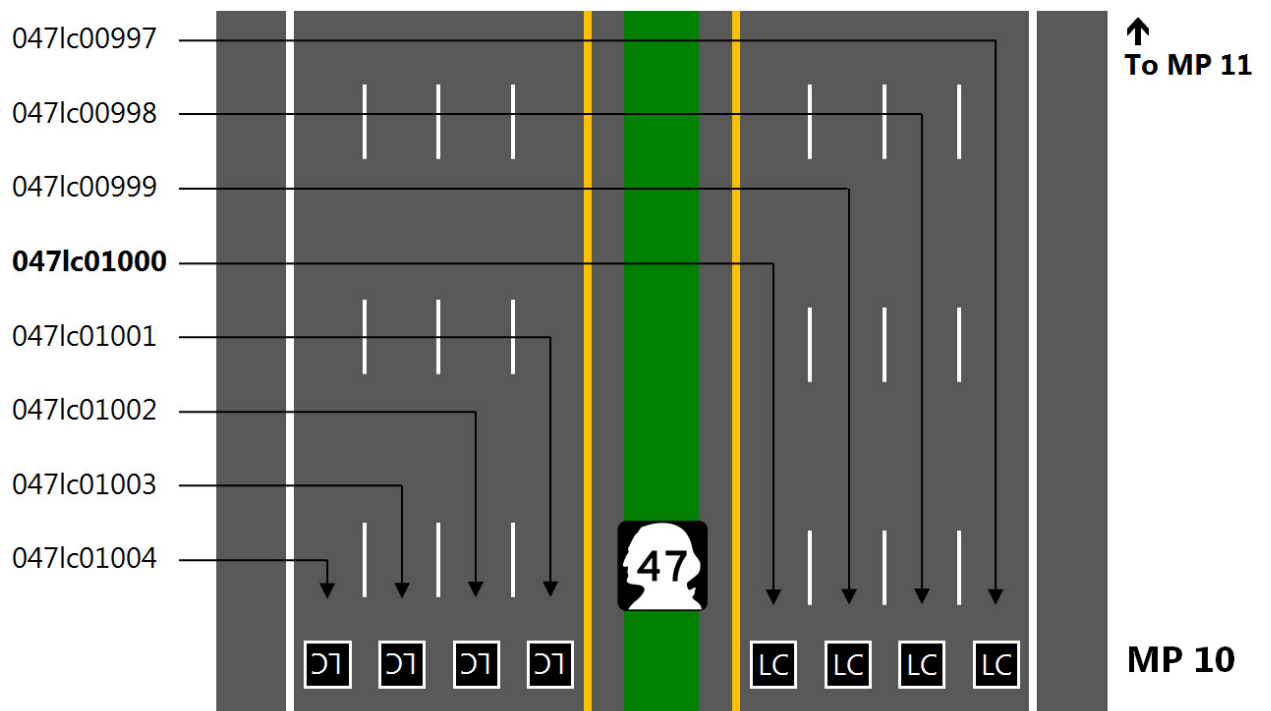
Figure 1-3: Example of lane control sign names on state highway 47
