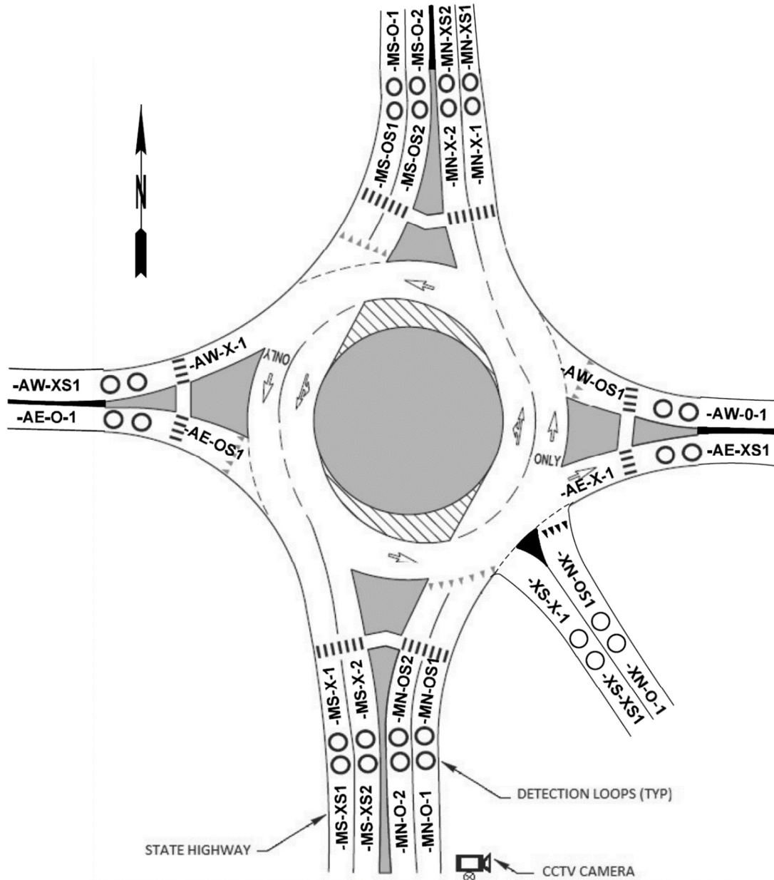
Figure 9-1: Loop naming scheme for roundabouts
